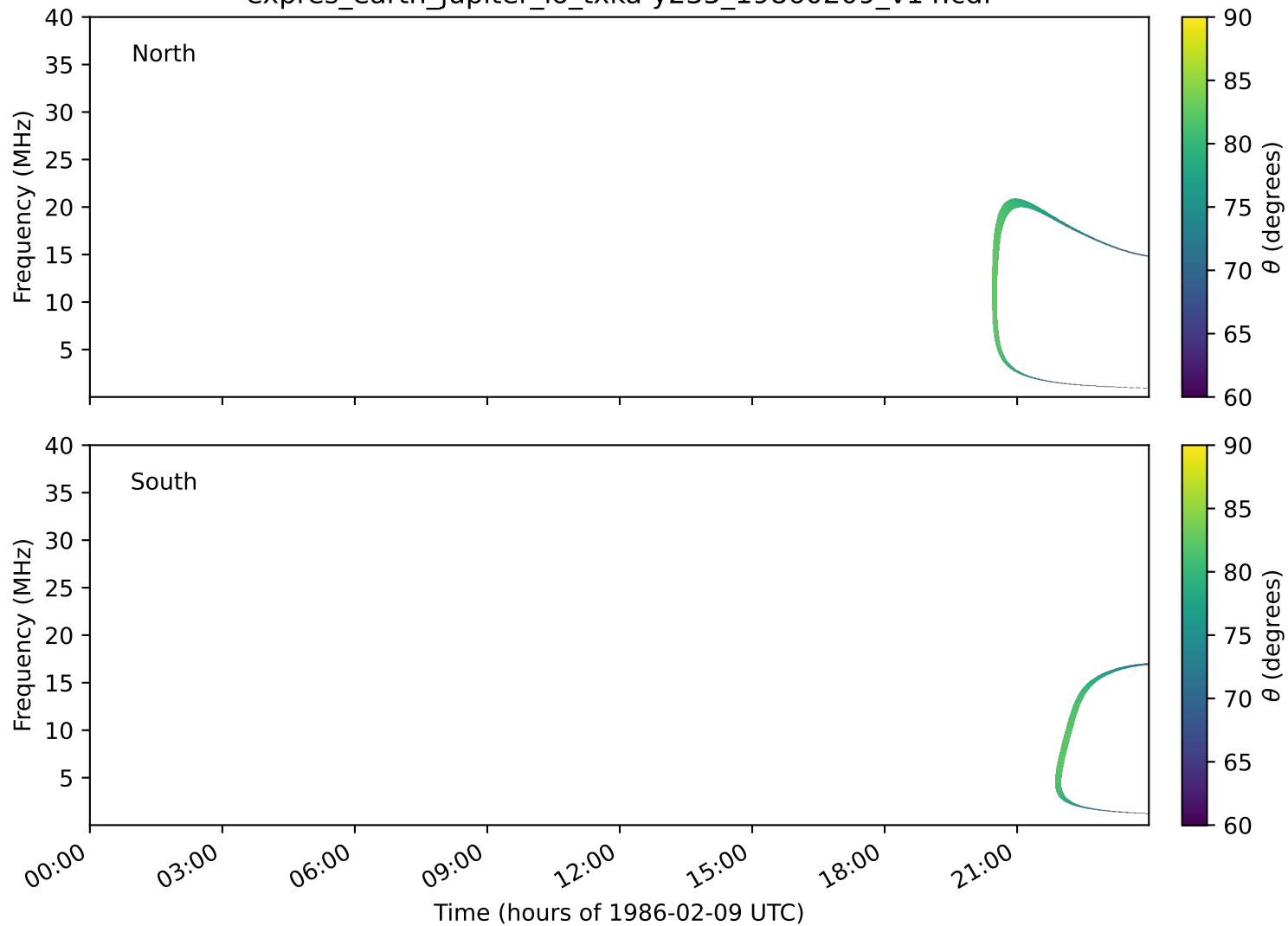
expres_earth_jupiter_io_txka-y235_19860209_v14.cdf
