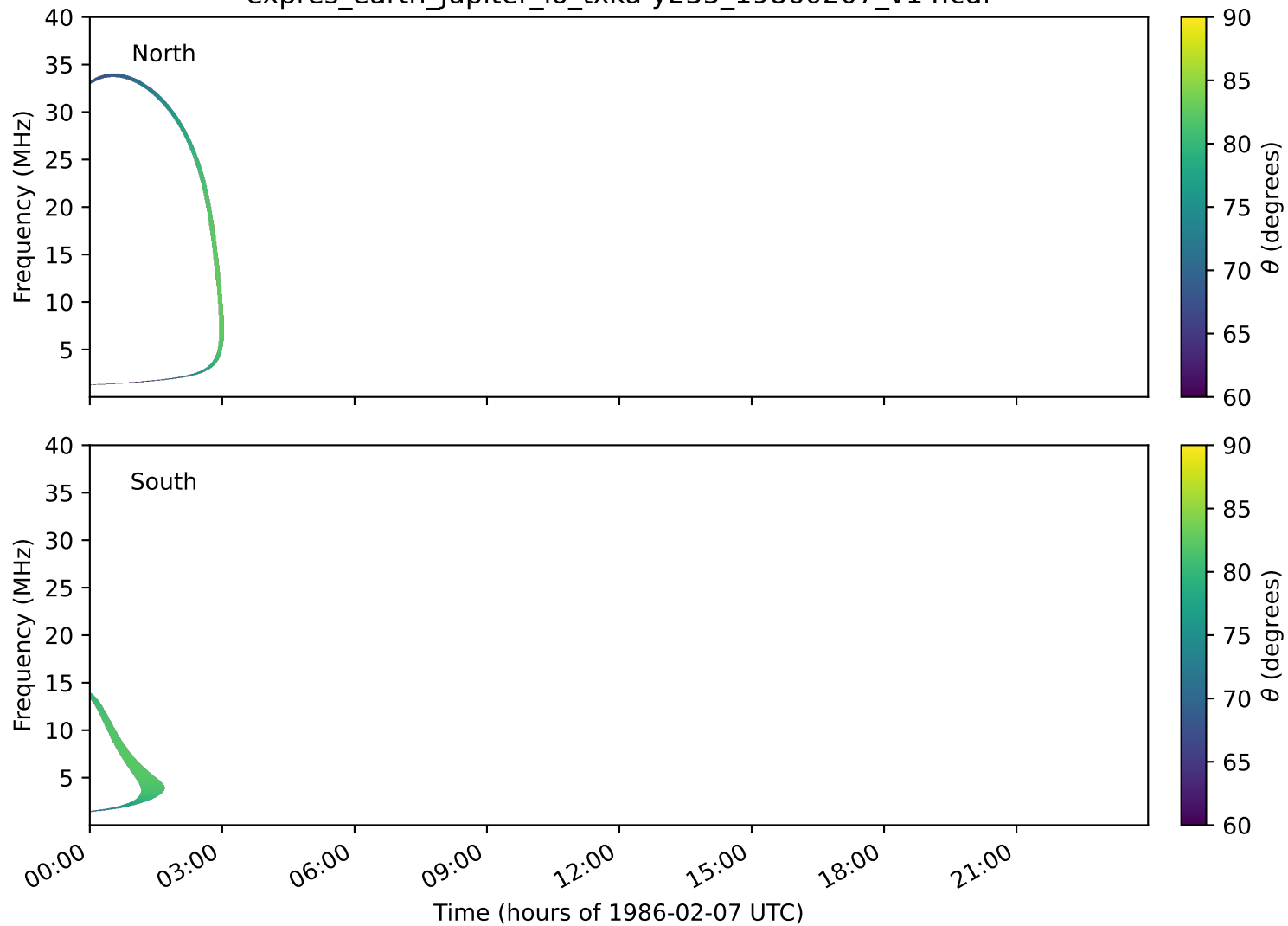
expres_earth_jupiter_io_txka-y235_19860207_v14.cdf
