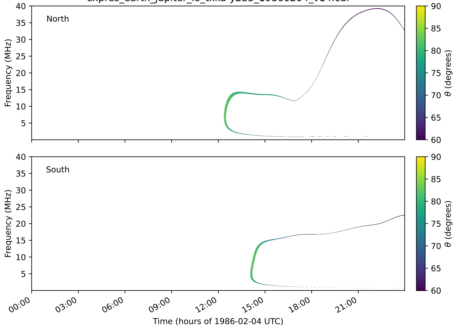
expres_earth_jupiter_io_txka-y235_19860204_v14.cdf
