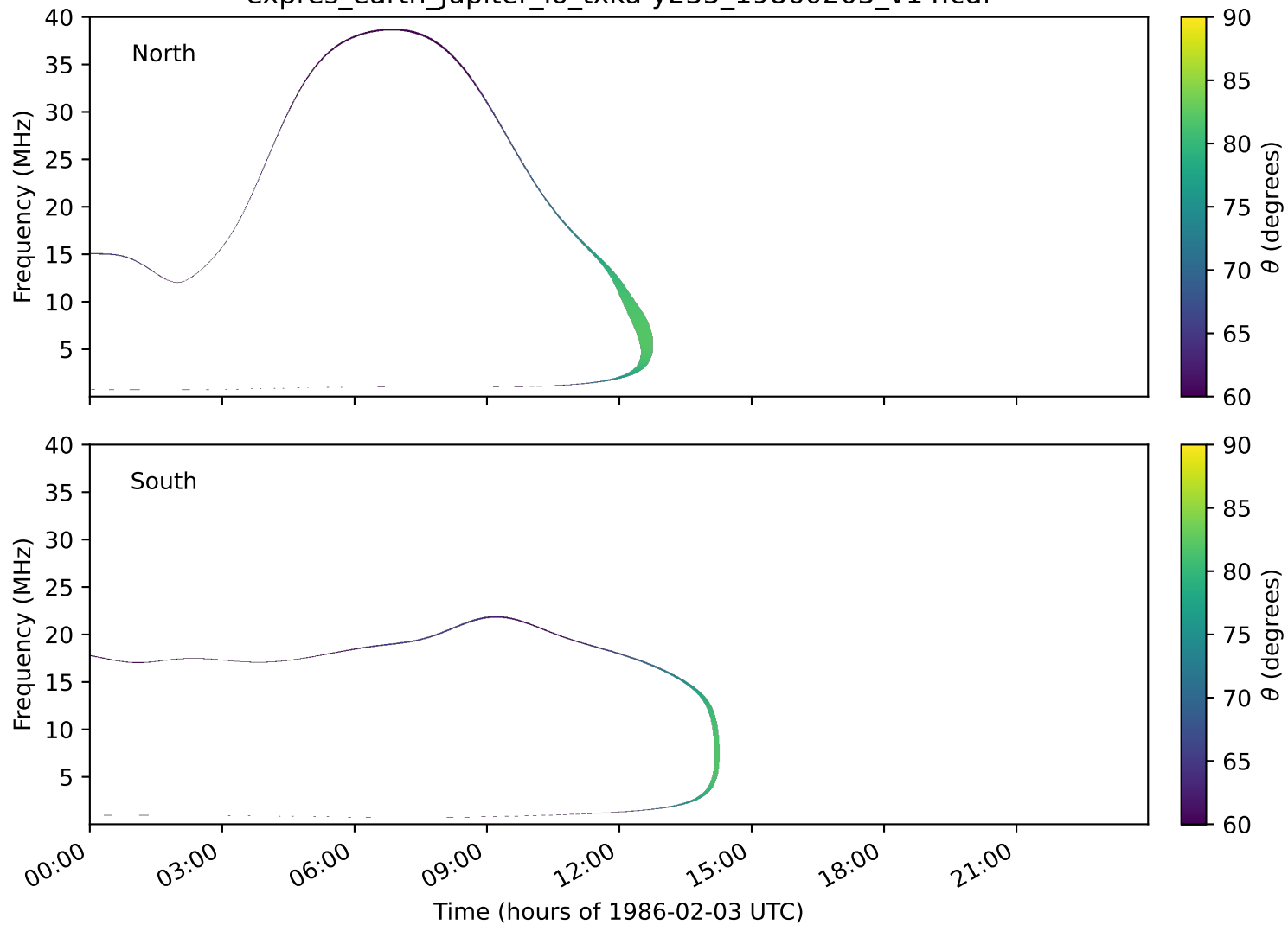
expres_earth_jupiter_io_txka-y235_19860203_v14.cdf
