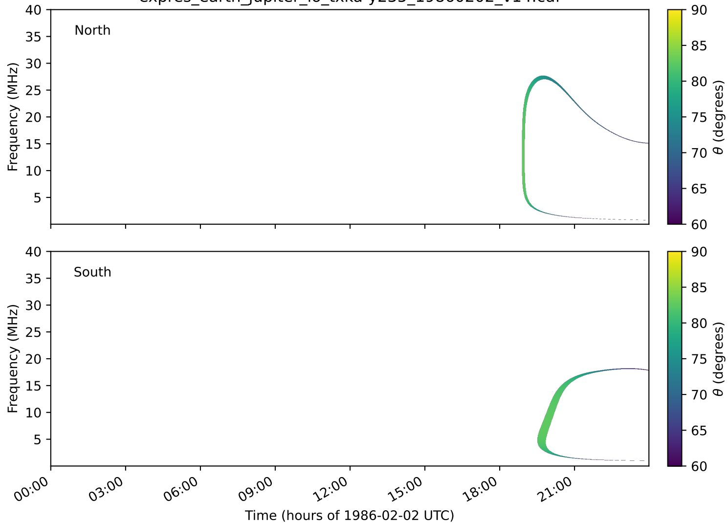
expres_earth_jupiter_io_txka-y235_19860202_v14.cdf
