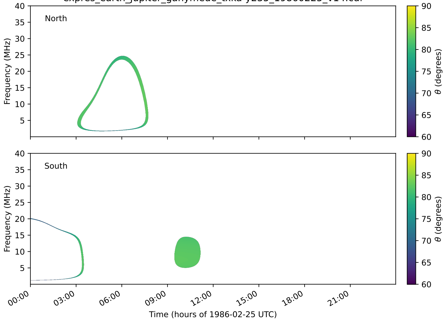
expres_earth_jupiter_ganymede_txka-y235_19860225_v14.cdf
