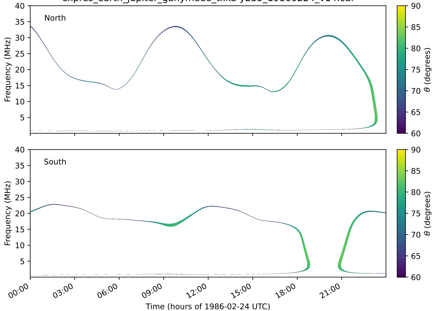
expres_earth_jupiter_ganymede_txka-y235_19860224_v14.cdf
