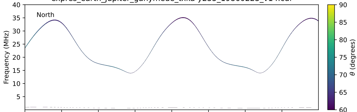
expres_earth_jupiter_ganymede_txka-y235_19860223_v14.cdf
