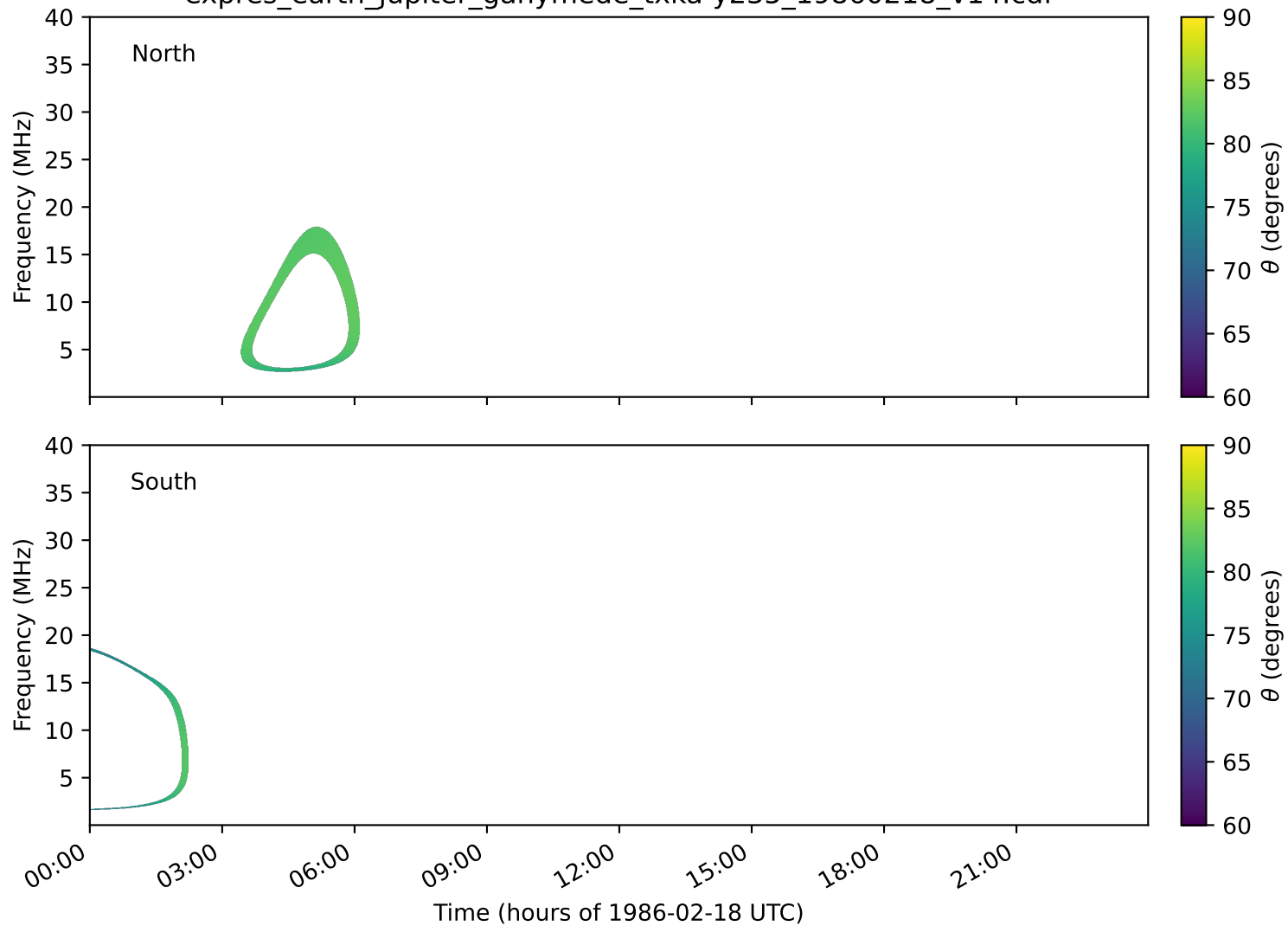
expres_earth_jupiter_ganymede_txka-y235_19860218_v14.cdf
