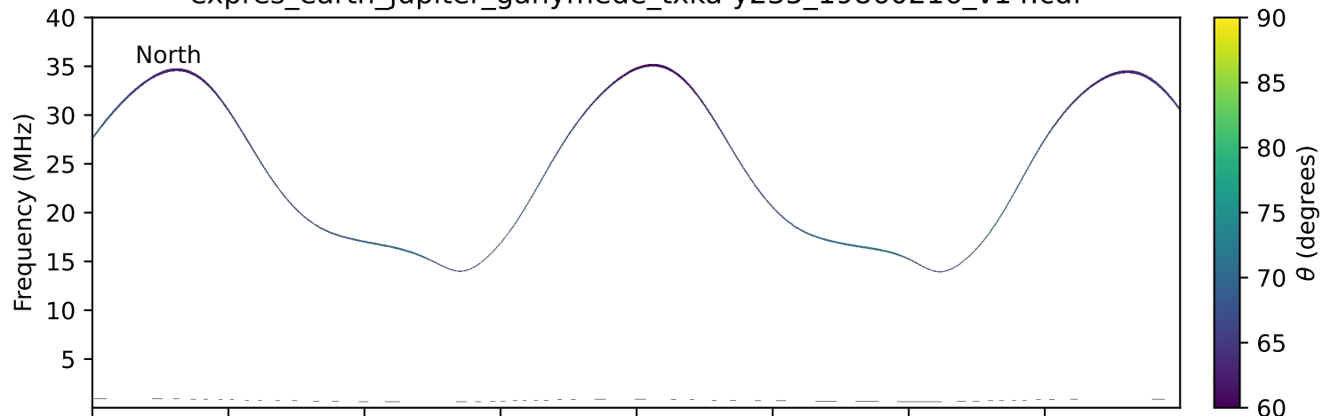
expres_earth_jupiter_ganymede_txka-y235_19860216_v14.cdf
