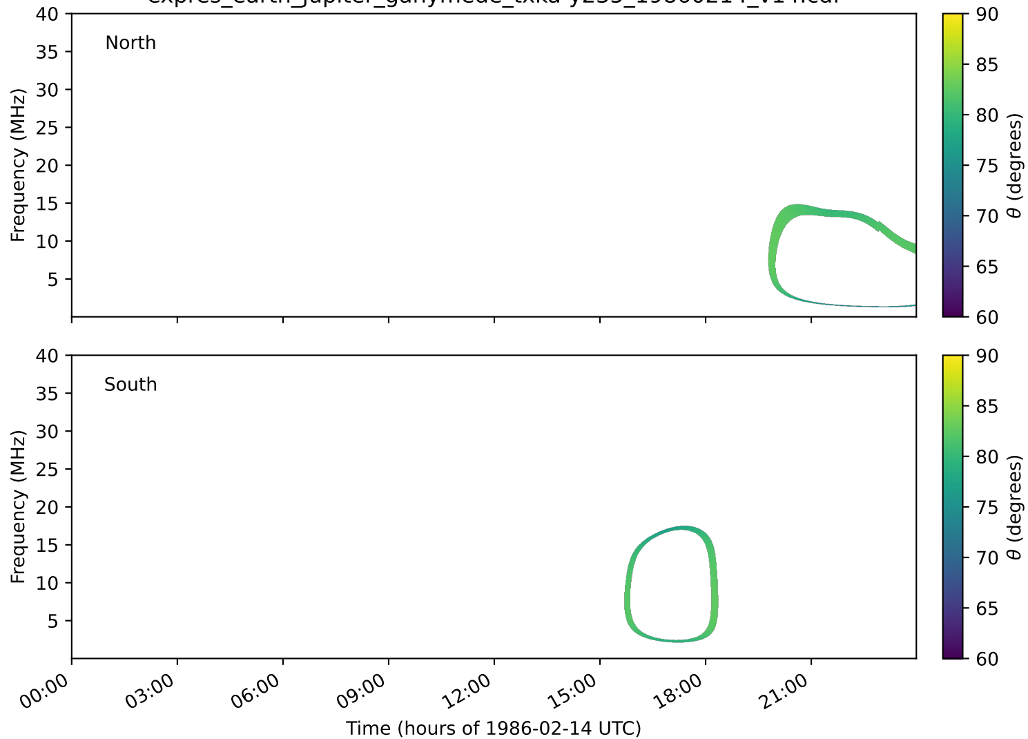
expres_earth_jupiter_ganymede_txka-y235_19860214_v14.cdf
