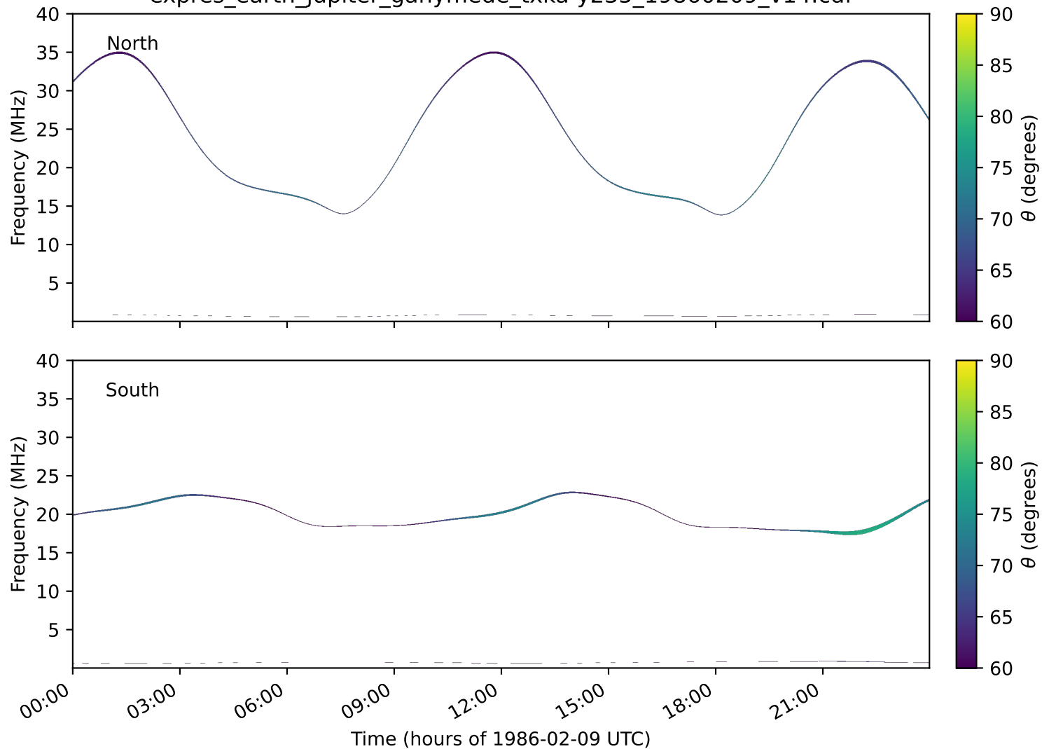
expres_earth_jupiter_ganymede_txka-y235_19860209_v14.cdf
