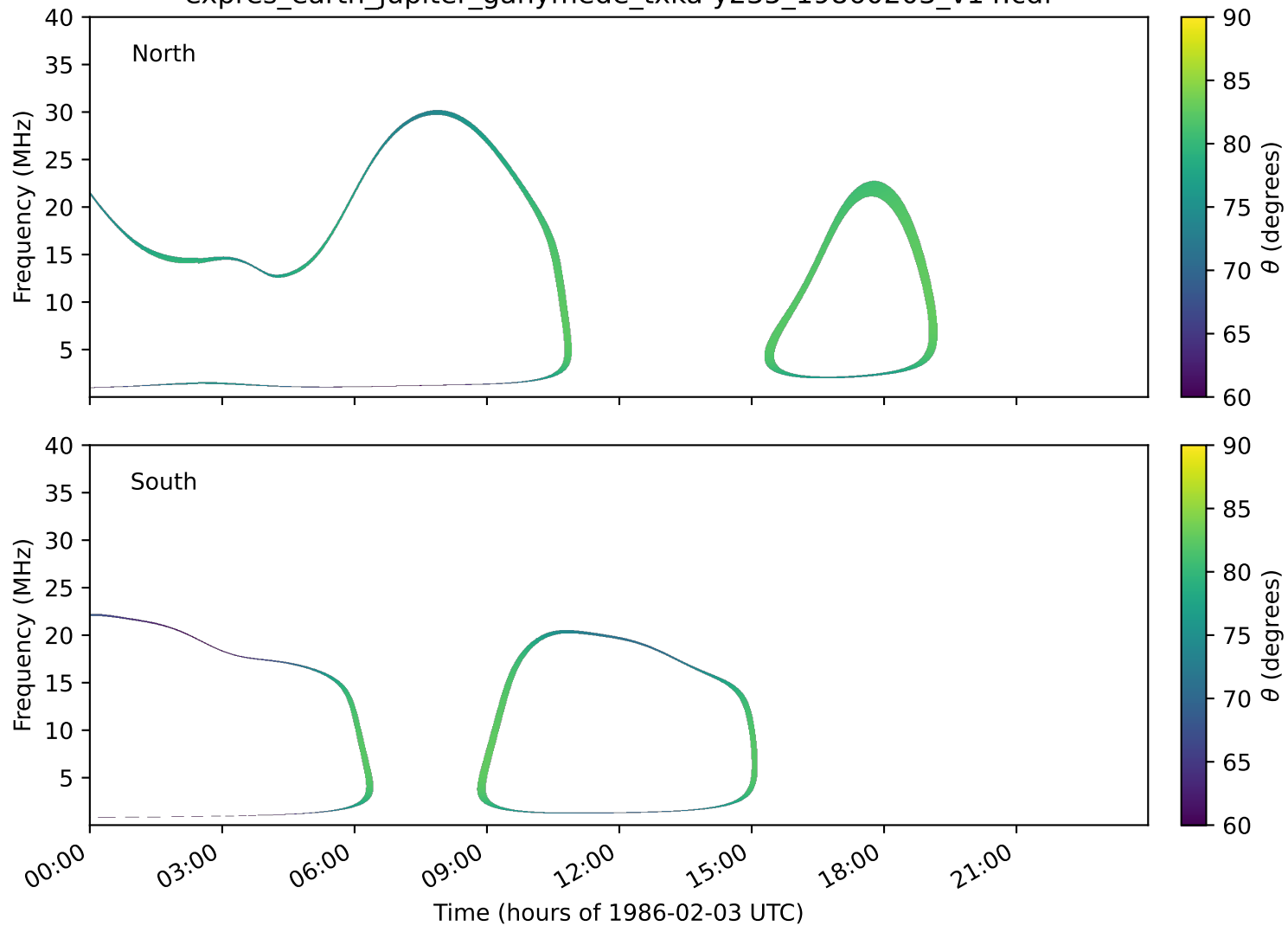
expres_earth_jupiter_ganymede_txka-y235_19860203_v14.cdf
