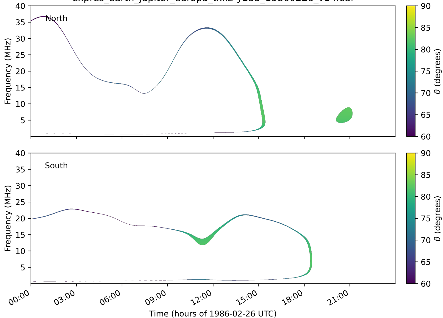
expres_earth_jupiter_europa_txka-y235_19860226_v14.cdf
