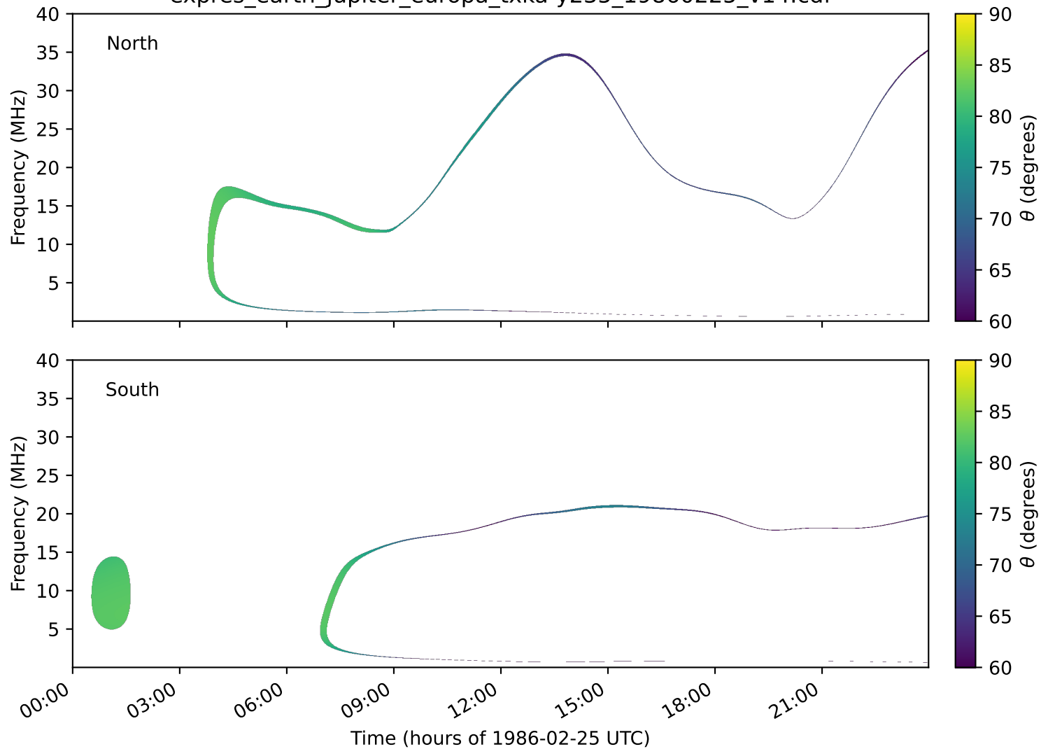
expres_earth_jupiter_europa_txka-y235_19860225_v14.cdf
