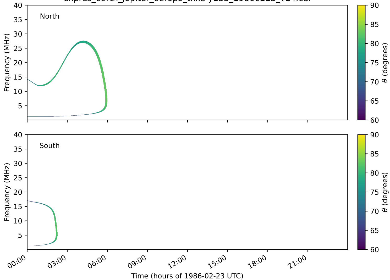
expres_earth_jupiter_europa_txka-y235_19860223_v14.cdf
