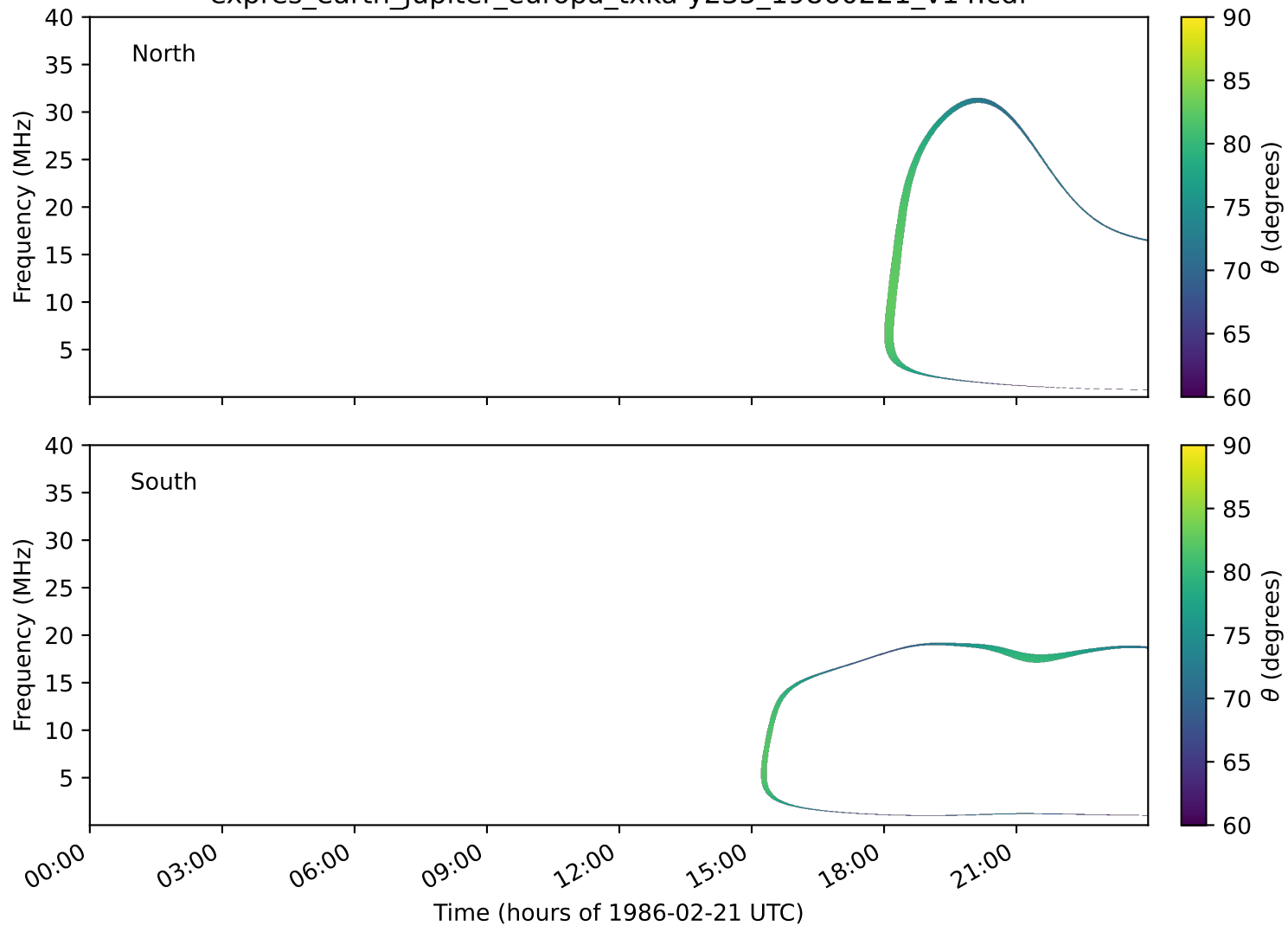
expres_earth_jupiter_europa_txka-y235_19860221_v14.cdf
