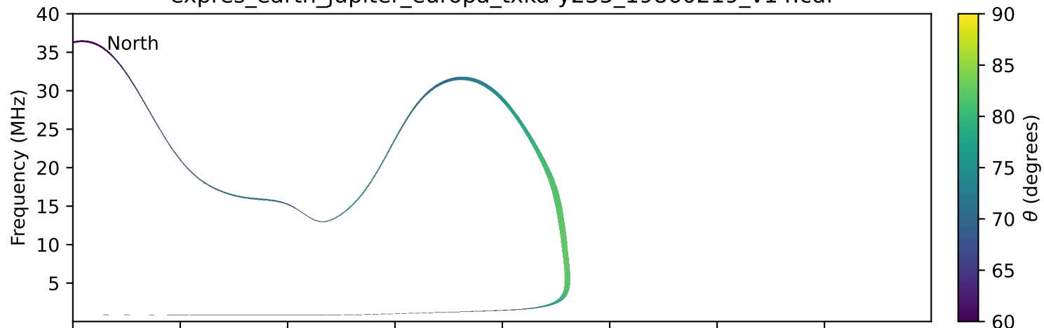
expres_earth_jupiter_europa_txka-y235_19860219_v14.cdf
