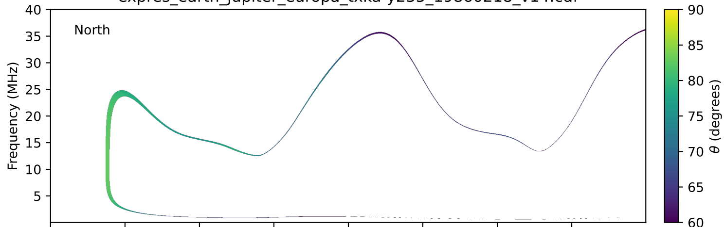
expres_earth_jupiter_europa_txka-y235_19860218_v14.cdf
