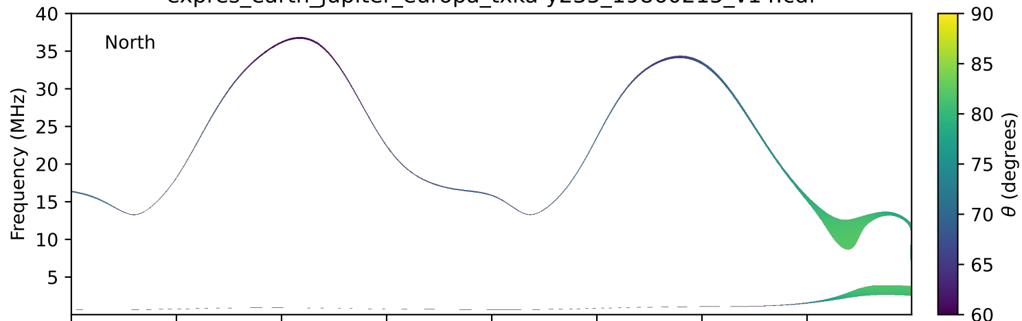
expres_earth_jupiter_europa_txka-y235_19860215_v14.cdf
