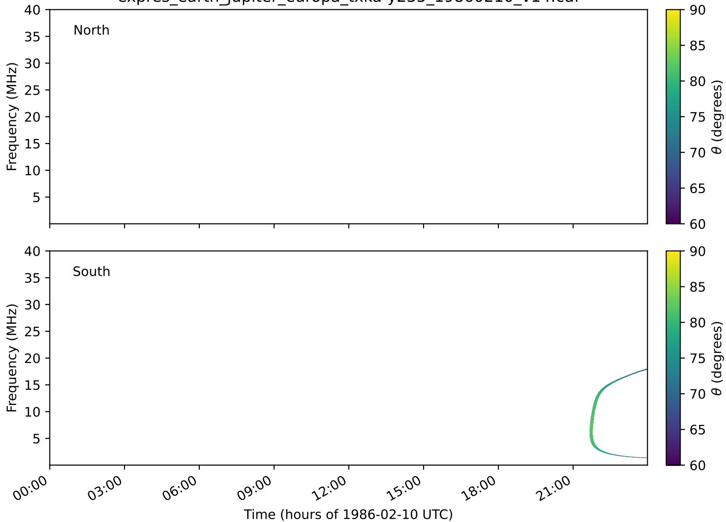
expres_earth_jupiter_europa_txka-y235_19860210_v14.cdf
