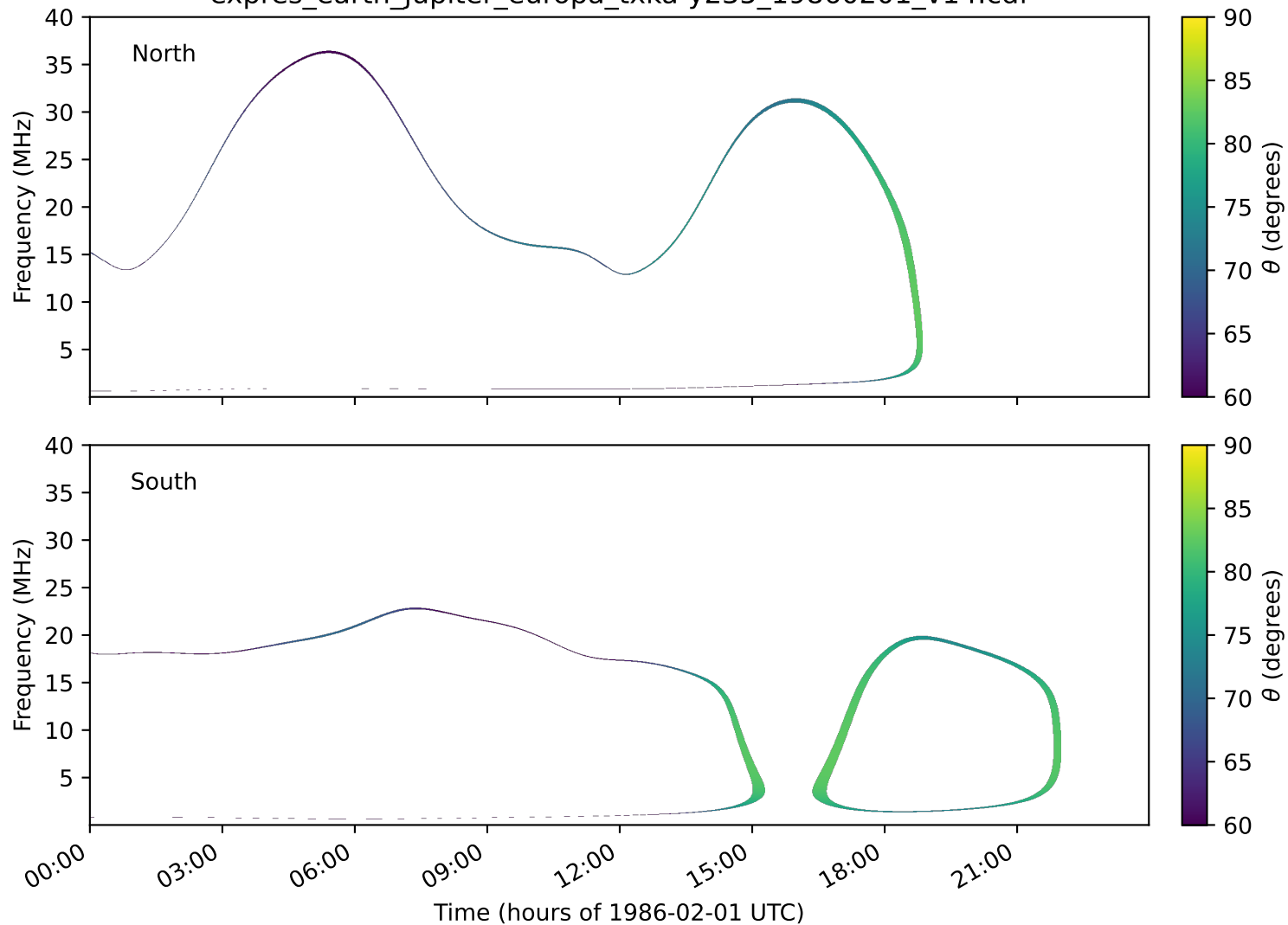
expres_earth_jupiter_europa_txka-y235_19860201_v14.cdf
