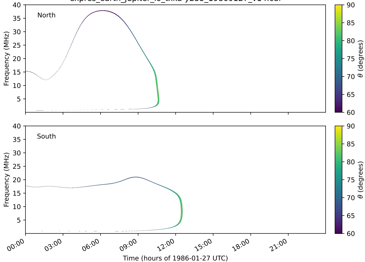
expres_earth_jupiter_io_txka-y235_19860127_v14.cdf
