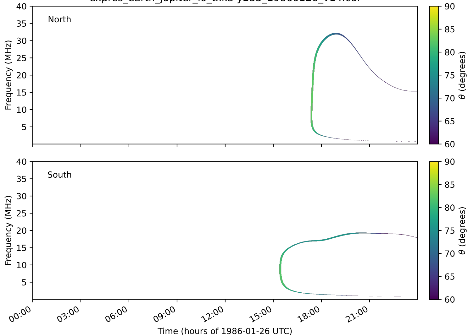
expres_earth_jupiter_io_txka-y235_19860126_v14.cdf
