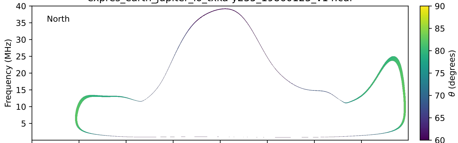
expres_earth_jupiter_io_txka-y235_19860123_v14.cdf
