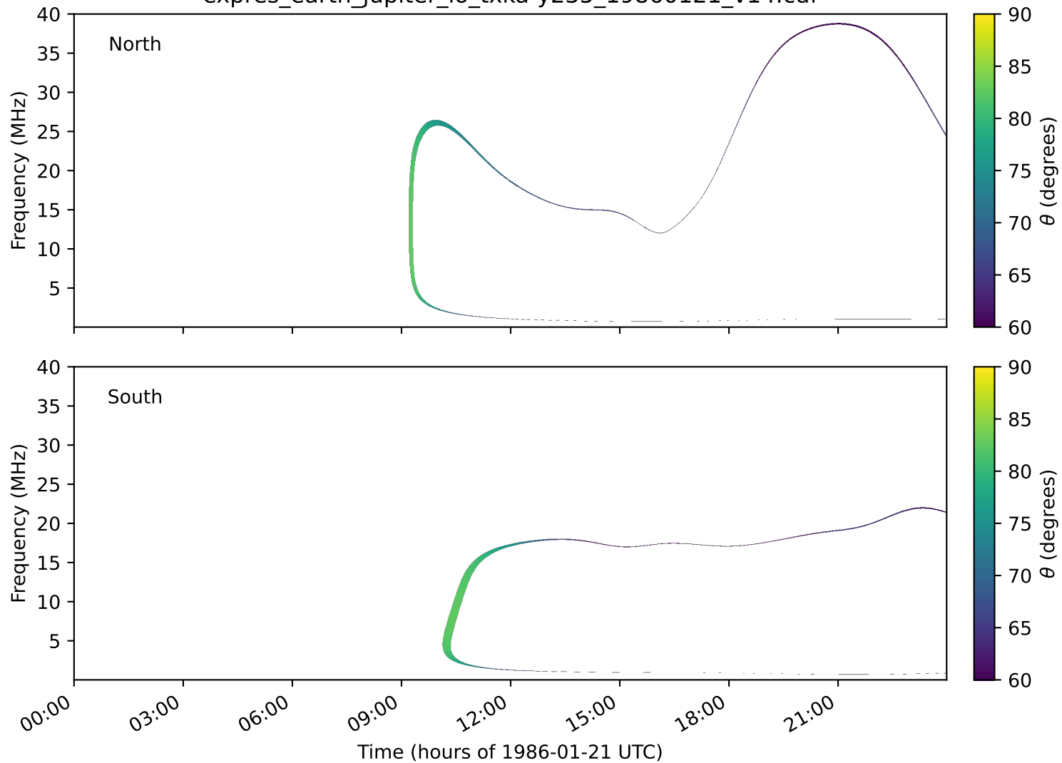
expres_earth_jupiter_io_txka-y235_19860121_v14.cdf
