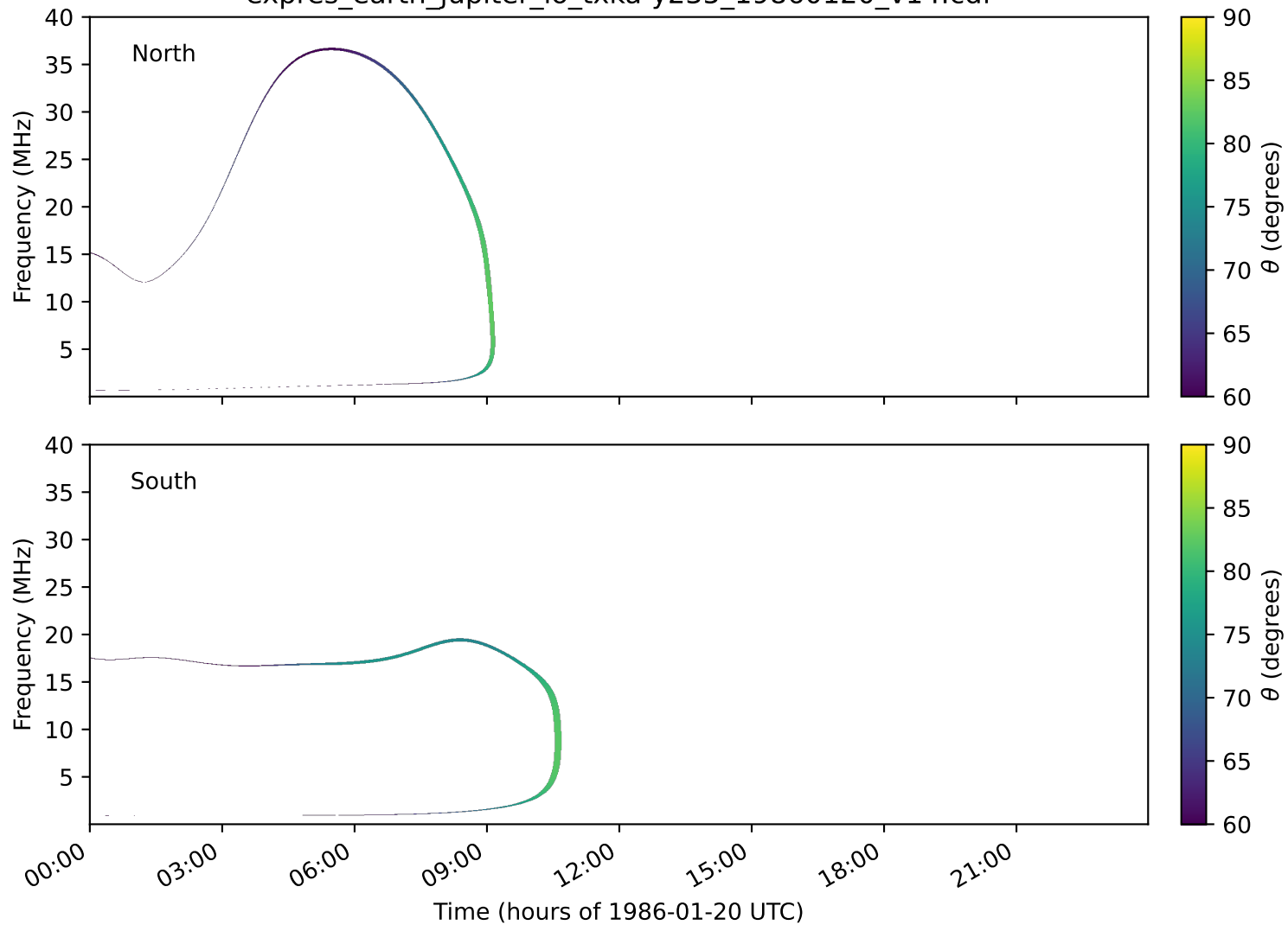
expres_earth_jupiter_io_txka-y235_19860120_v14.cdf
