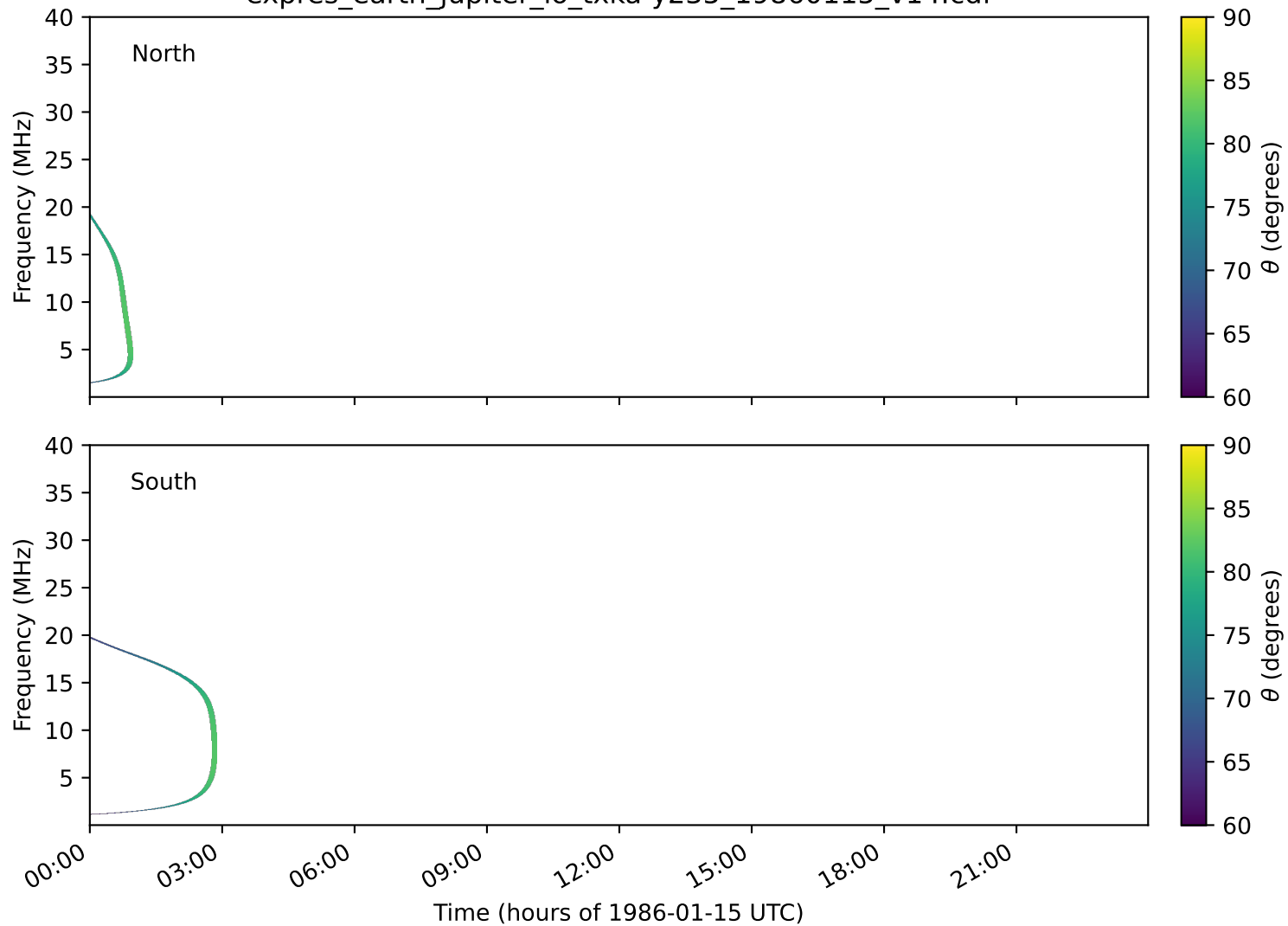
expres_earth_jupiter_io_txka-y235_19860115_v14.cdf
