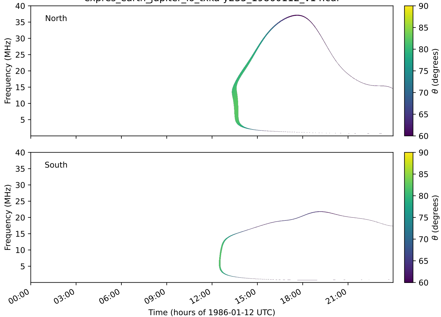
expres_earth_jupiter_io_txka-y235_19860112_v14.cdf
