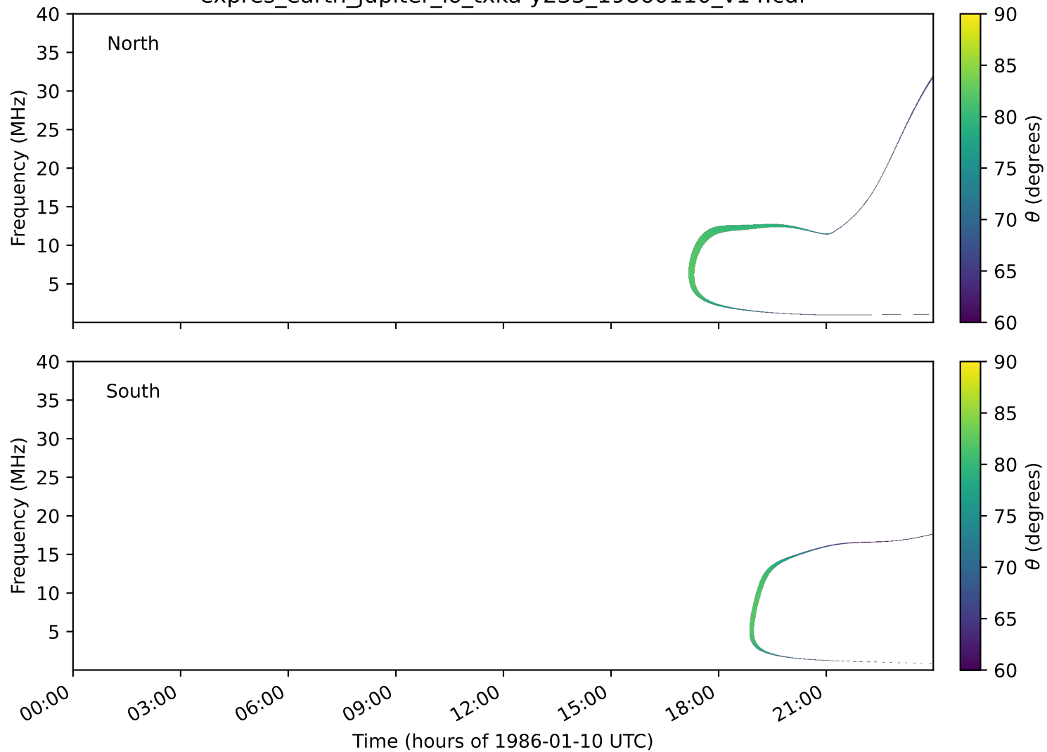
expres_earth_jupiter_io_txka-y235_19860110_v14.cdf
