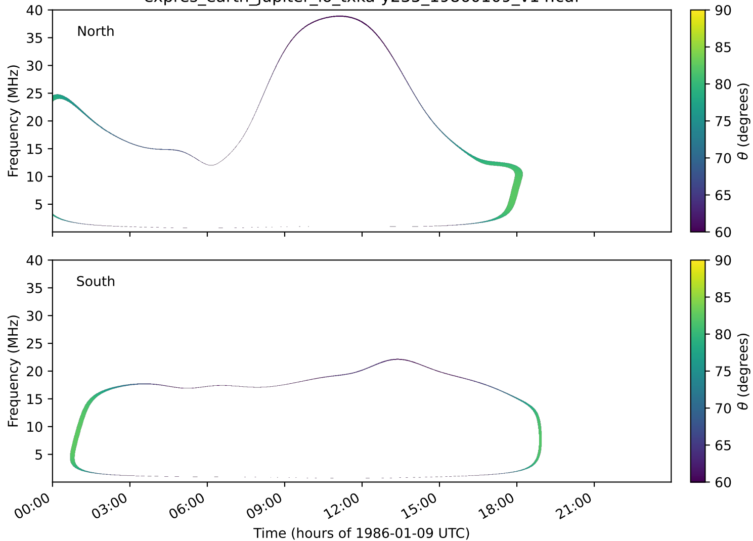
expres_earth_jupiter_io_txka-y235_19860109_v14.cdf
