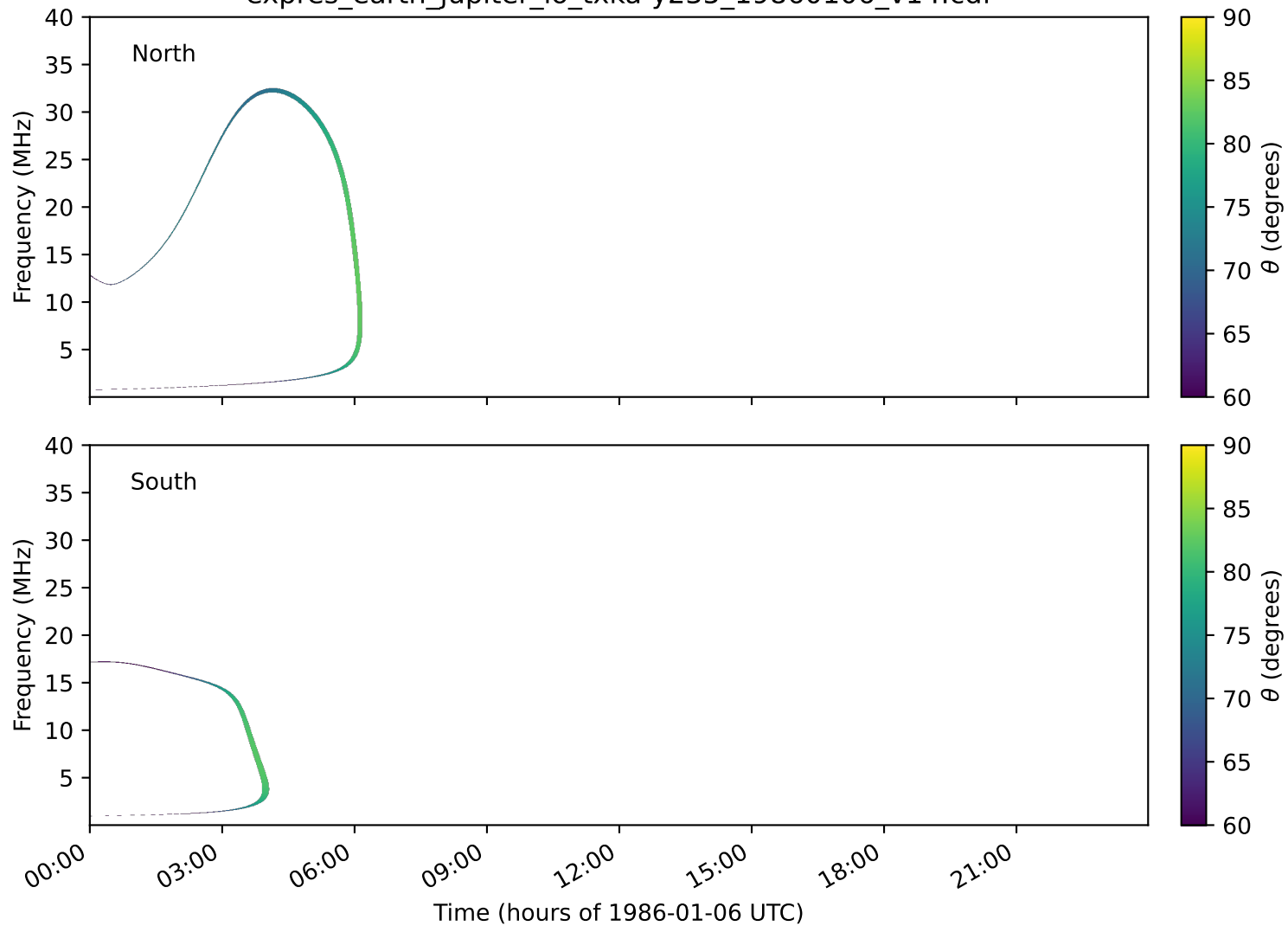
expres_earth_jupiter_io_txka-y235_19860106_v14.cdf
