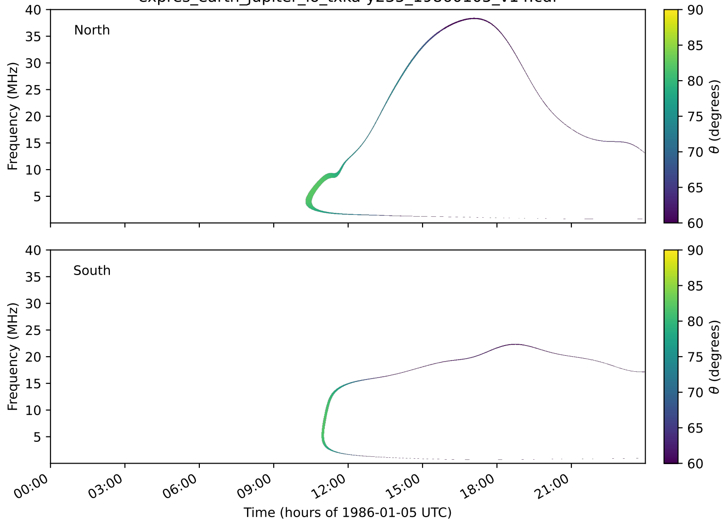
expres_earth_jupiter_io_txka-y235_19860105_v14.cdf
