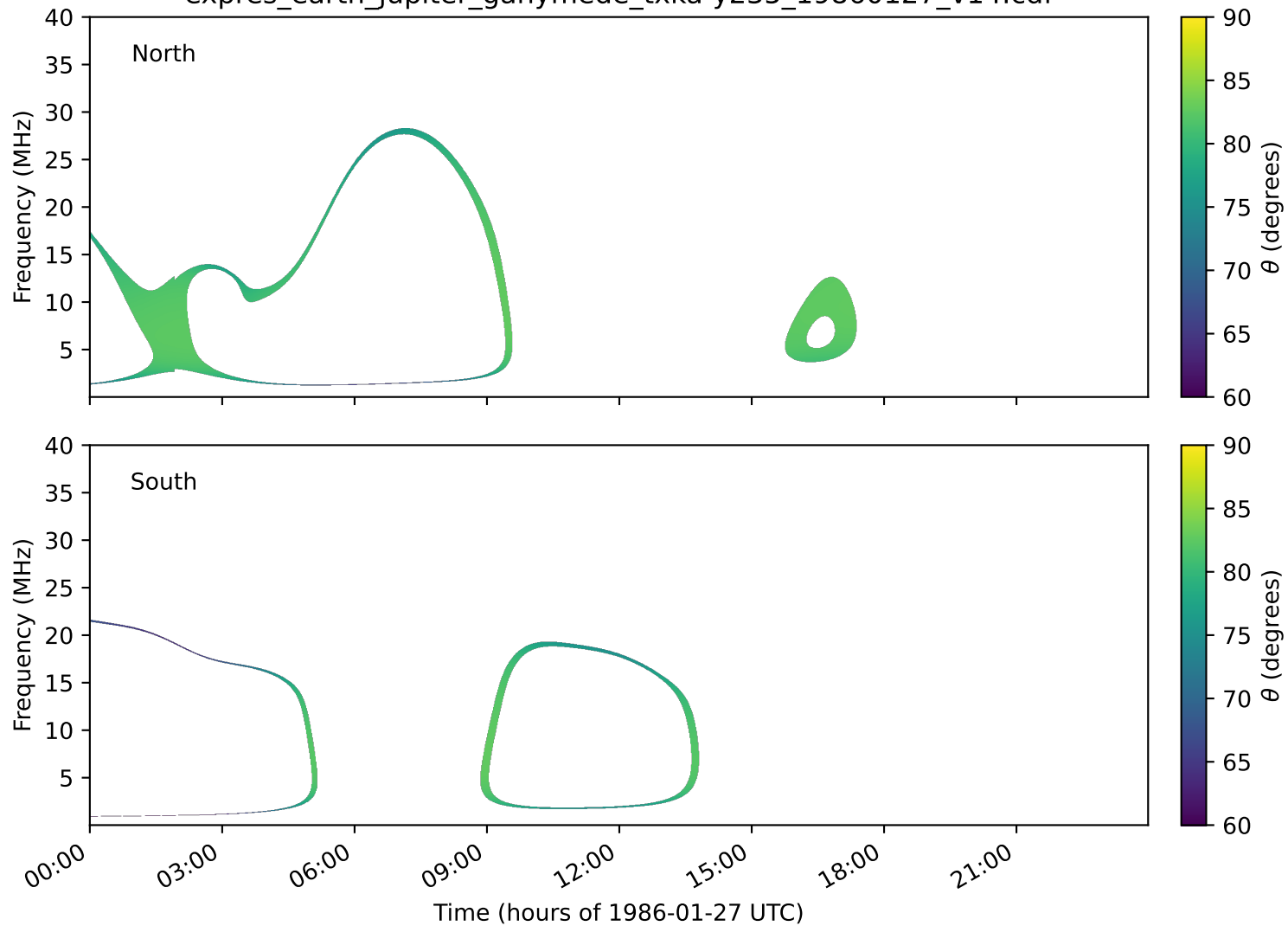
expres_earth_jupiter_ganymede_txka-y235_19860127_v14.cdf
