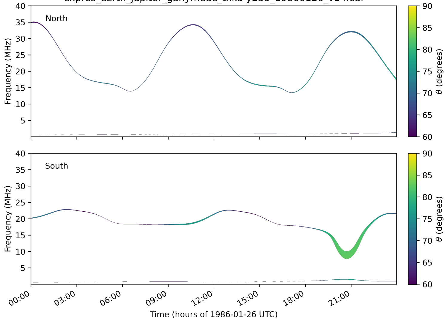
expres_earth_jupiter_ganymede_txka-y235_19860126_v14.cdf
