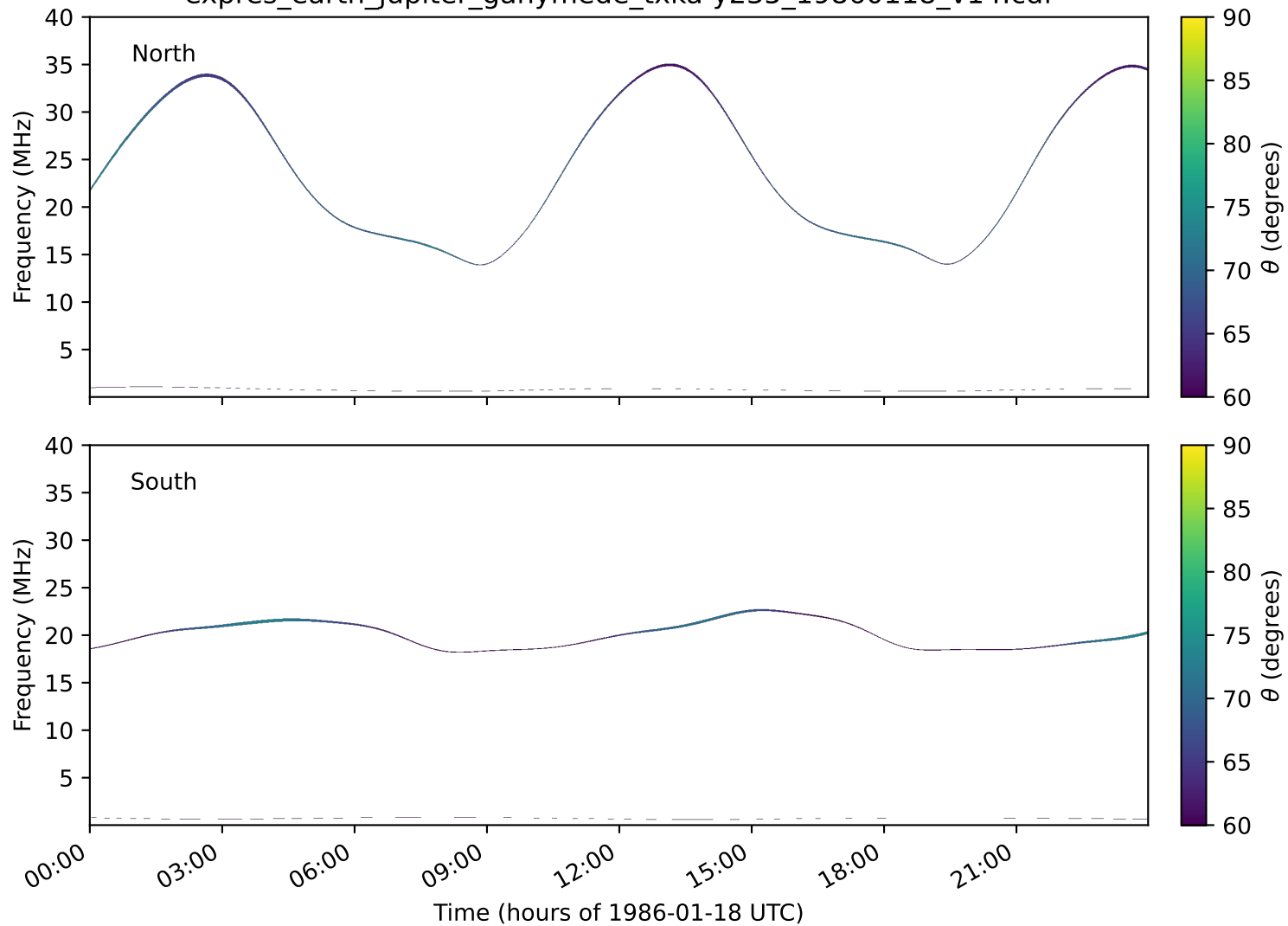
expres_earth_jupiter_ganymede_txka-y235_19860118_v14.cdf
