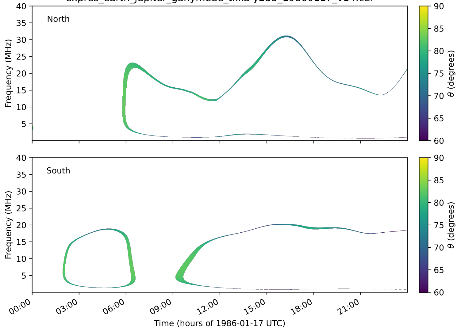
expres_earth_jupiter_ganymede_txka-y235_19860117_v14.cdf
