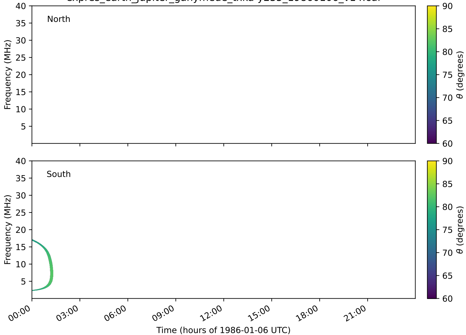
expres_earth_jupiter_ganymede_txka-y235_19860106_v14.cdf
