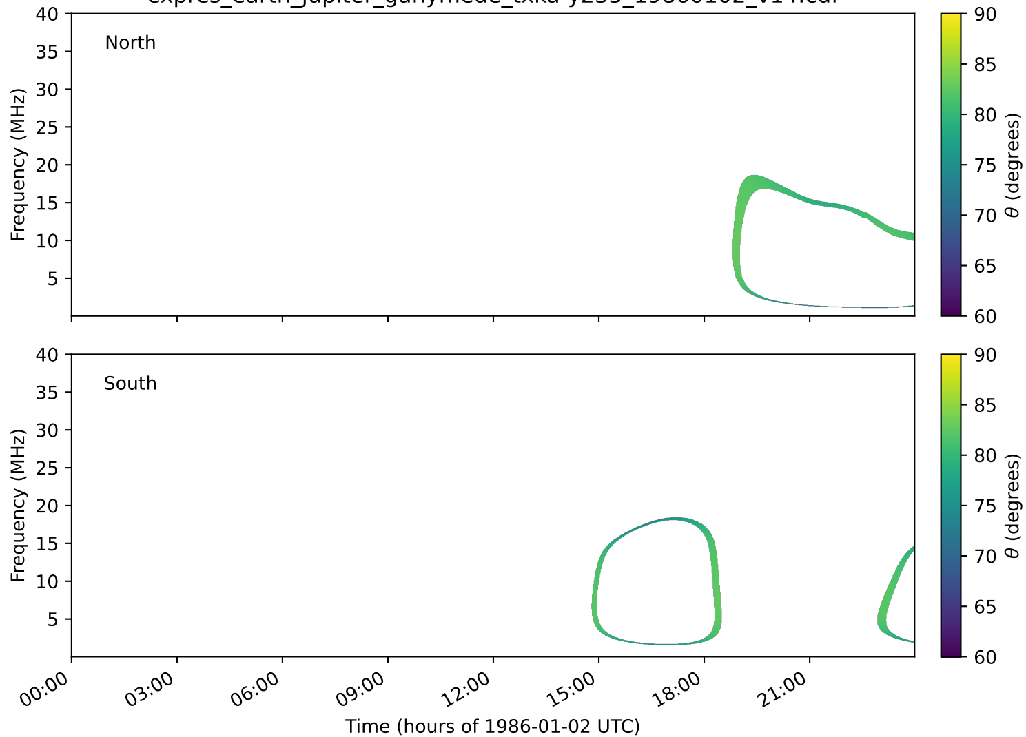
expres_earth_jupiter_ganymede_txka-y235_19860102_v14.cdf
