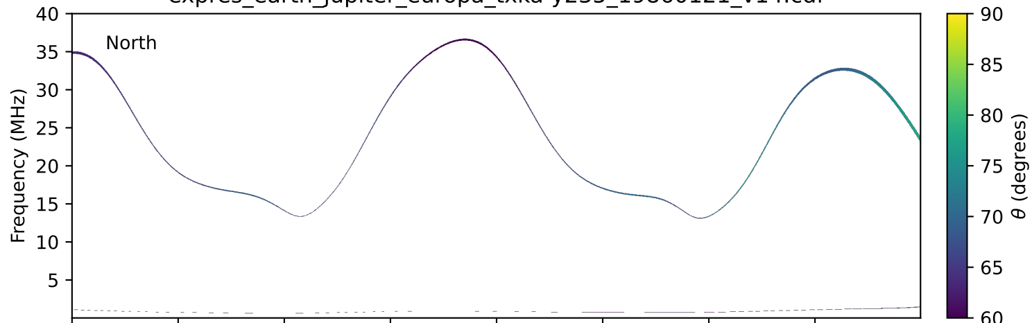
expres_earth_jupiter_europa_txka-y235_19860121_v14.cdf
