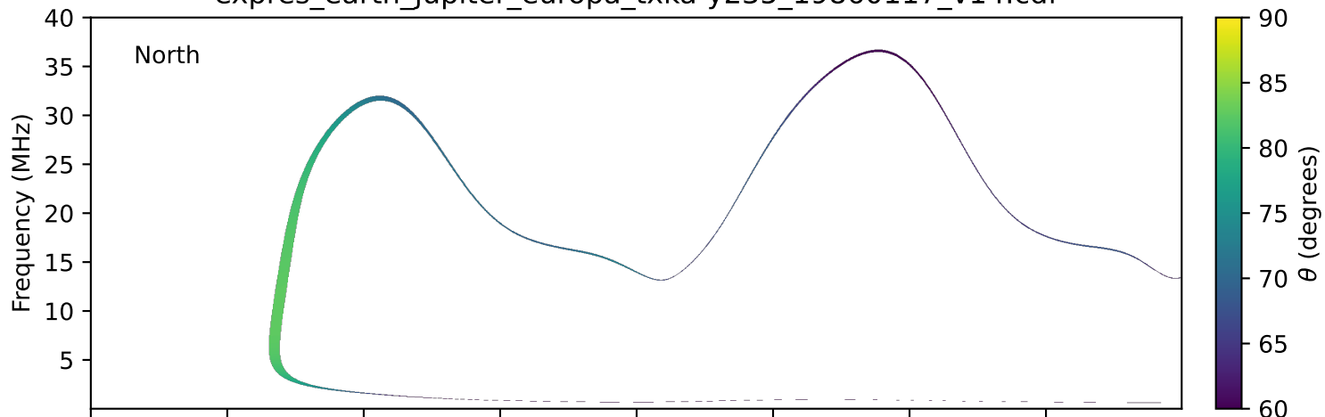
expres_earth_jupiter_europa_txka-y235_19860117_v14.cdf
