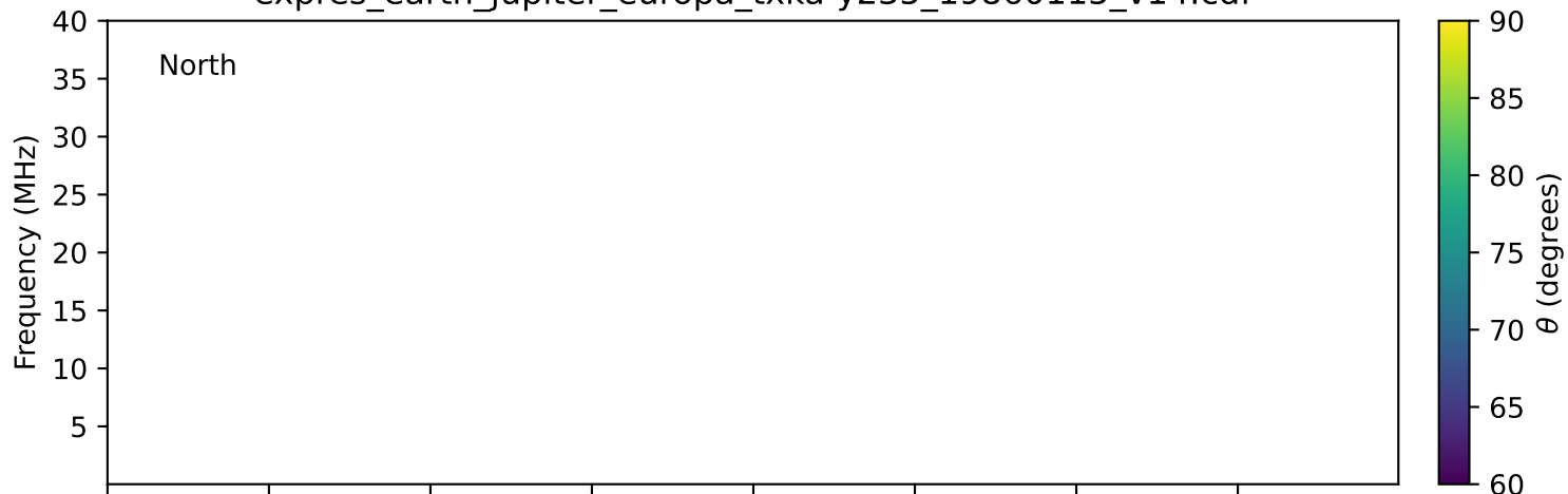
expres_earth_jupiter_europa_txka-y235_19860115_v14.cdf
