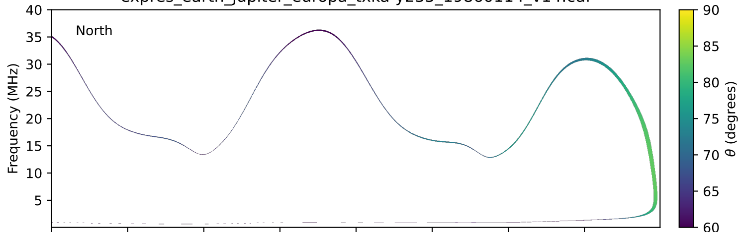
expres_earth_jupiter_europa_txka-y235_19860114_v14.cdf
