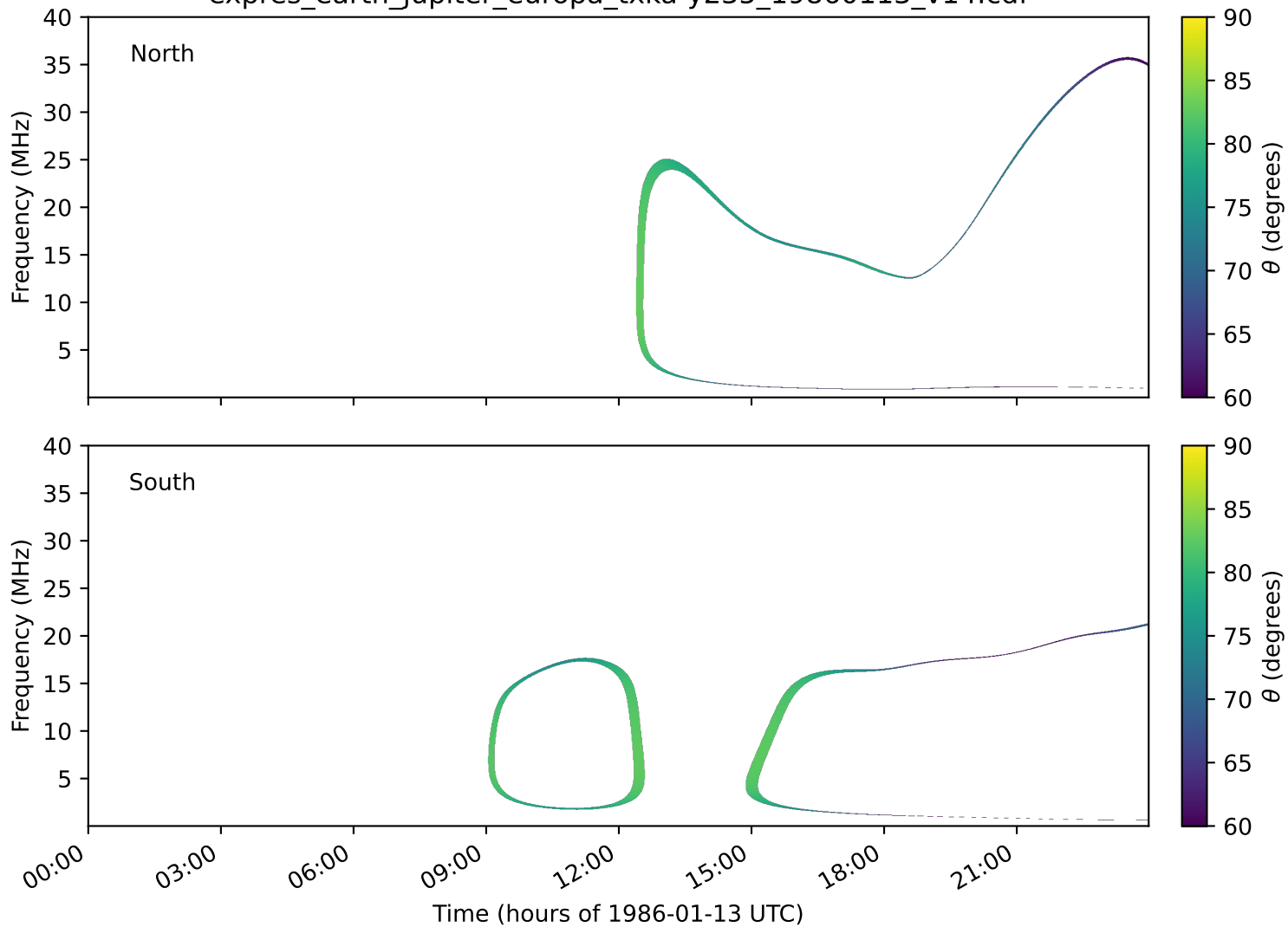
expres_earth_jupiter_europa_txka-y235_19860113_v14.cdf
