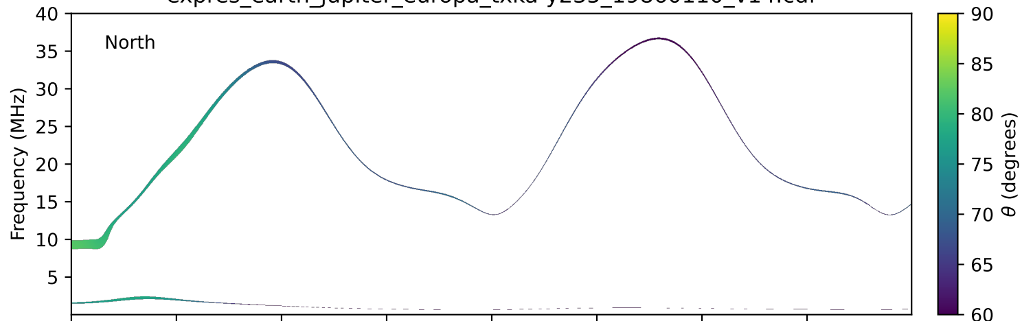
expres_earth_jupiter_europa_txka-y235_19860110_v14.cdf
