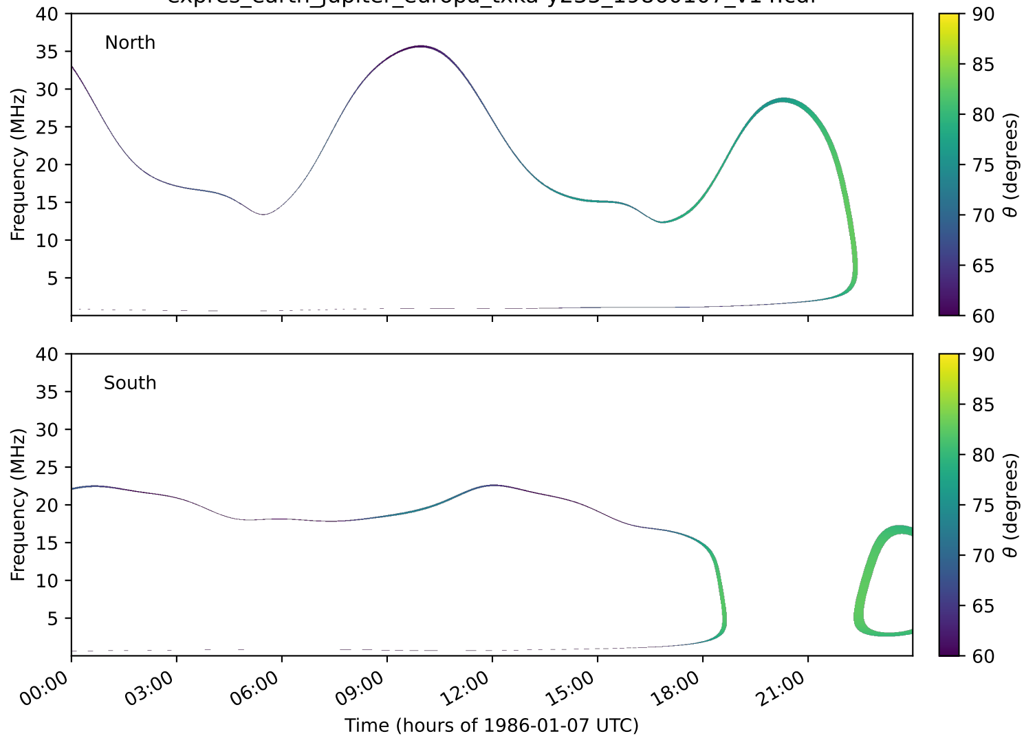
expres_earth_jupiter_europa_txka-y235_19860107_v14.cdf
