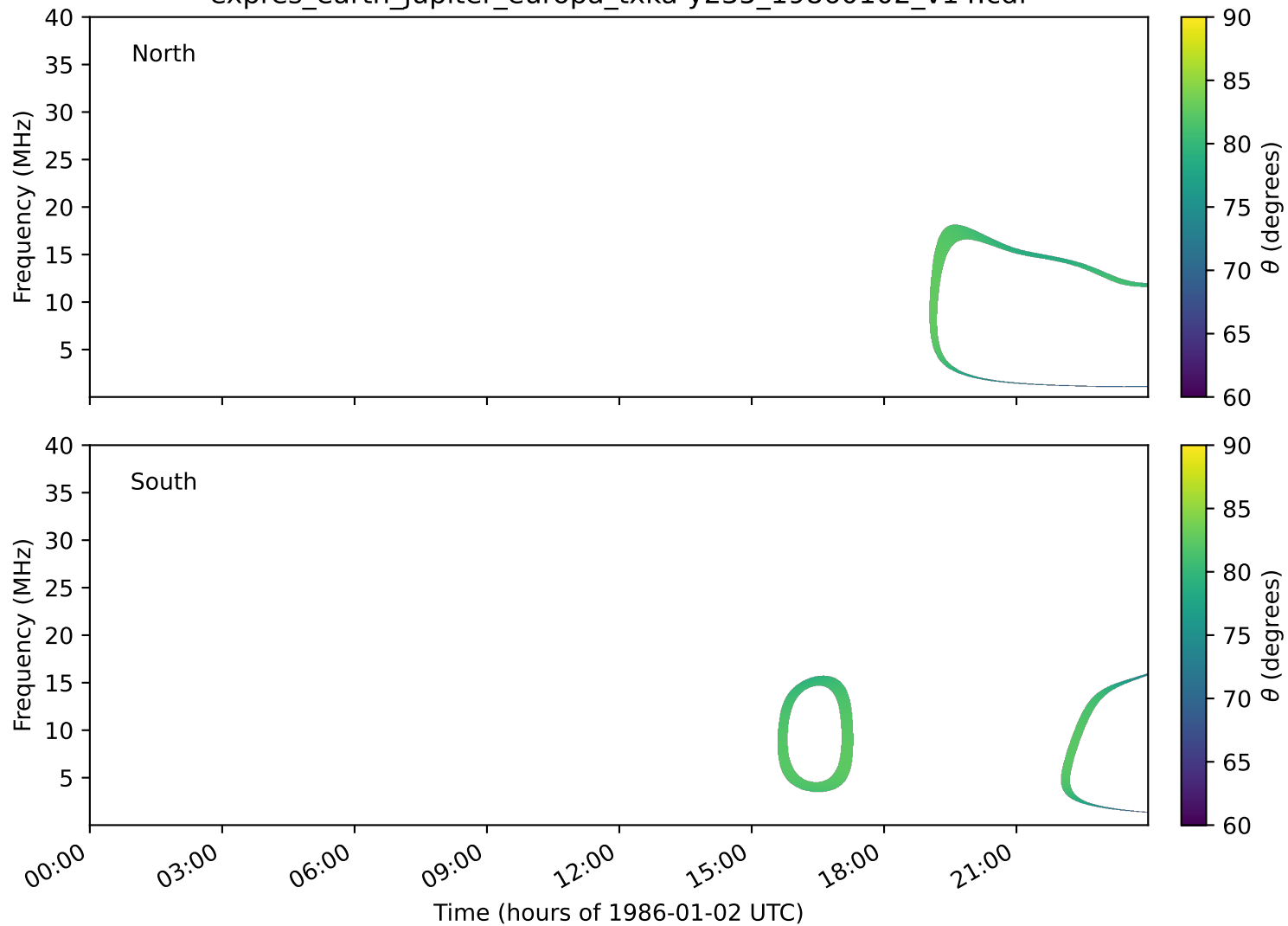
expres_earth_jupiter_europa_txka-y235_19860102_v14.cdf
