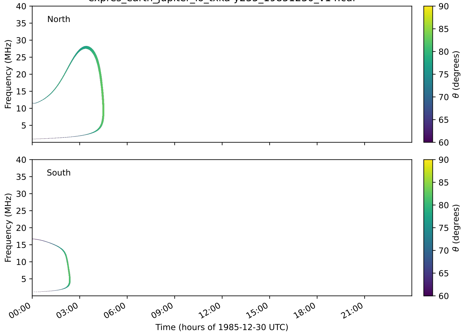
expres_earth_jupiter_io_txka-y235_19851230_v14.cdf
