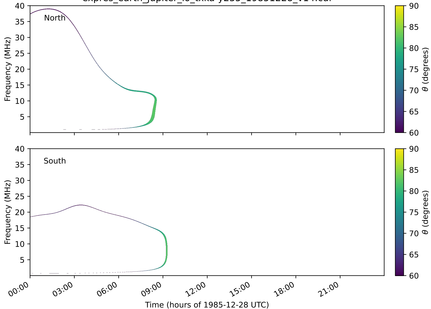
expres_earth_jupiter_io_txka-y235_19851228_v14.cdf
