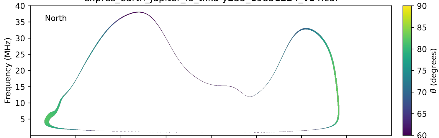
expres_earth_jupiter_io_txka-y235_19851224_v14.cdf
